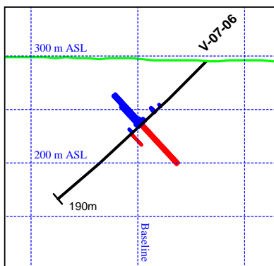
Cross section 1675S Hole V-07-06
