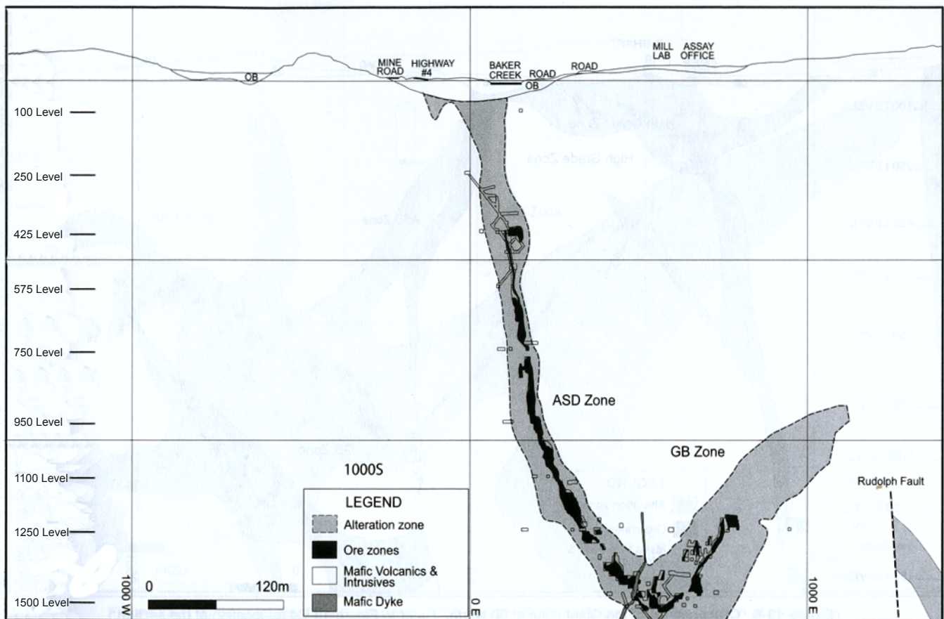
Figure 4a: Cross-section of the Giant mine at 1000 South.
