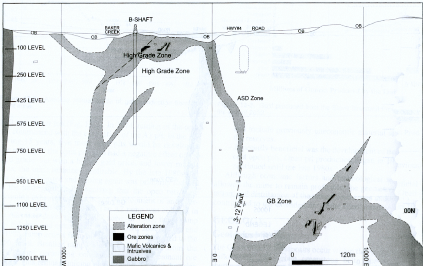
Figure 4b: Cross-section of the Giant mine at 00 North
