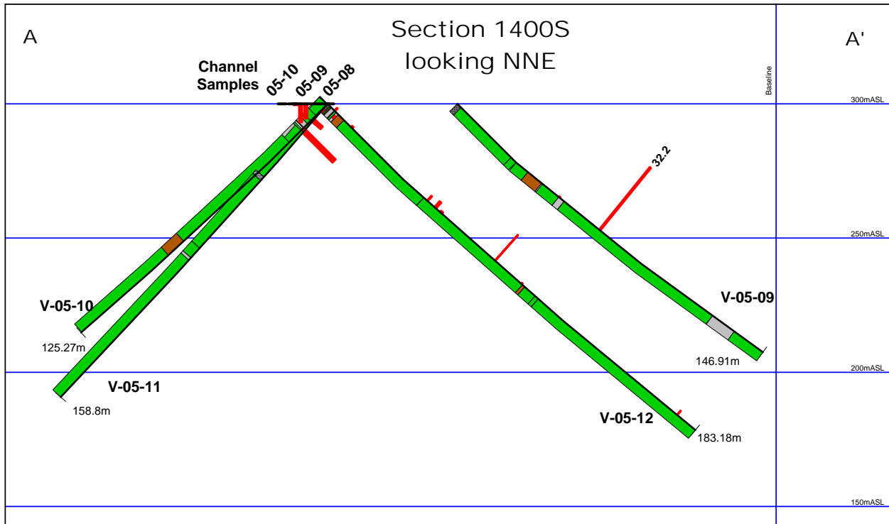
FIGURE 5 DRILL SECTIONS
